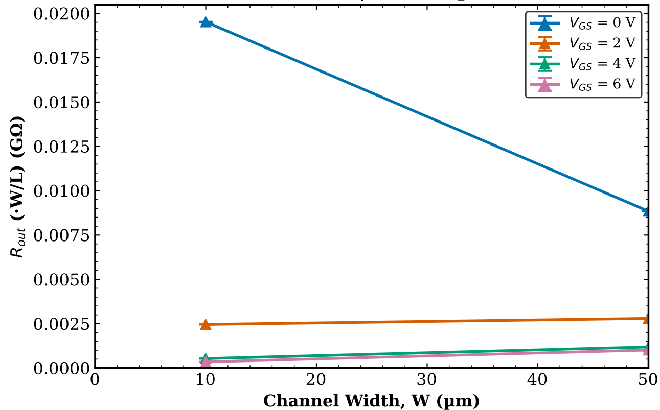
TFT2 Transistor 1 R_{out} vs W | L = 20\text{ }\mu\text{m}
